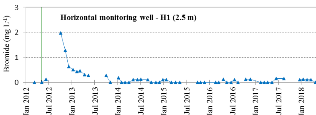
Figure 3.5. Bromide concentration in the groundwater at Jyndeved . The data derive from the horizontal monitoring well H1. The green vertical line indicates the date of bromide application.
