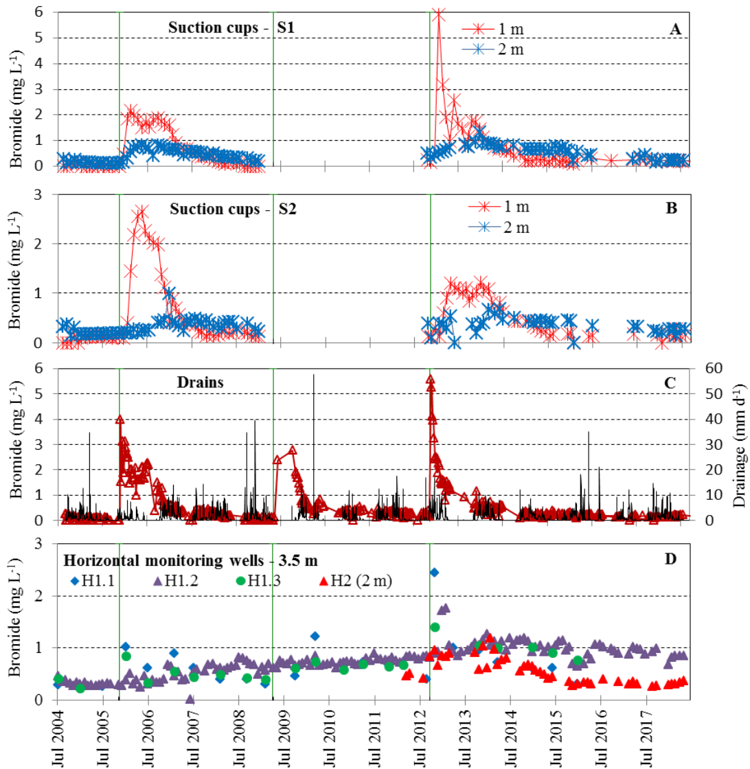
Figure 5.3. Bromide concentration at Estrup. A and B refer to suction cups located at S1 and S2, respectively. The bromide concentration is also shown for drainage runoff (C) and the horizontal monitoring well H1 and H2 (D). From September 2008 to August 2012, bromide measurements in the suction cups were suspended. The green vertical lines indicate the dates of bromide application.
