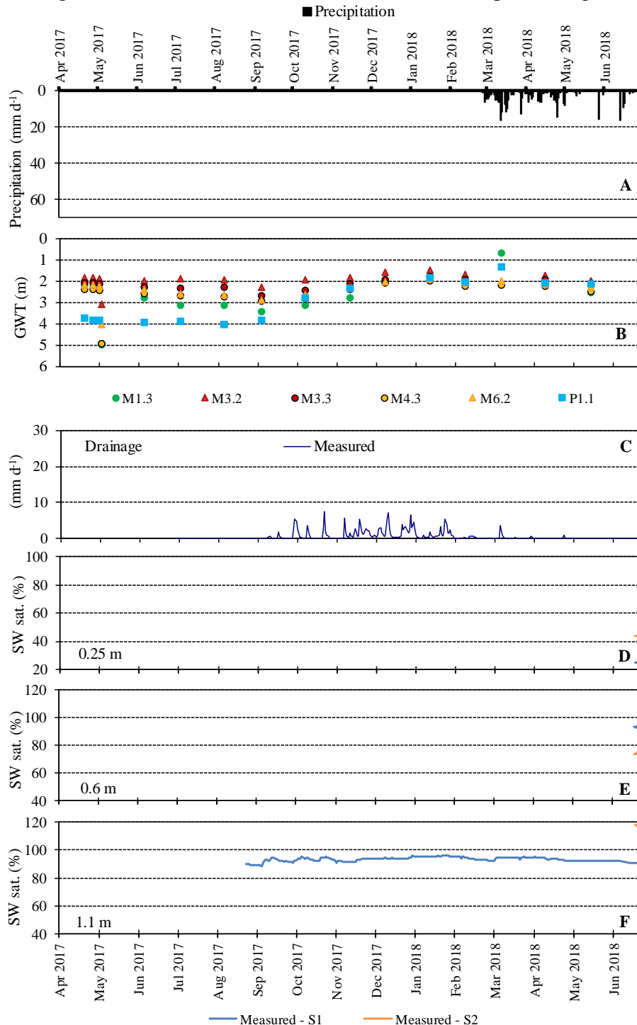
Figure 7.2. Soil water dynamics at Lund : Measured precipitation (A), measured groundwater table, GWT (B), measured drainage (C), and measured saturation (SW sat.) at three different soil depths (D, E and F). The measured data in B derived from piezometers located in the buffer zone. The measured data in D, E and F derived from TDR probes installed at S1 and S2 (Figure 7.1).
